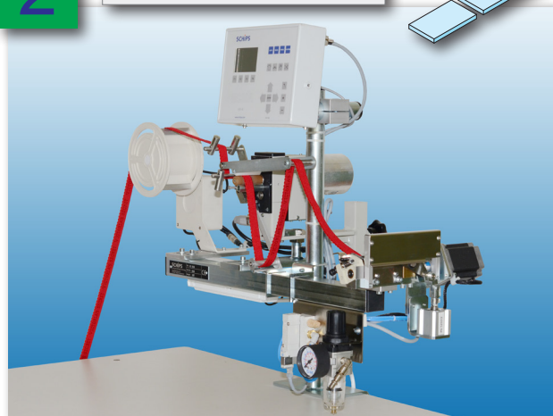
Tape cutting automat, compact and low cost
